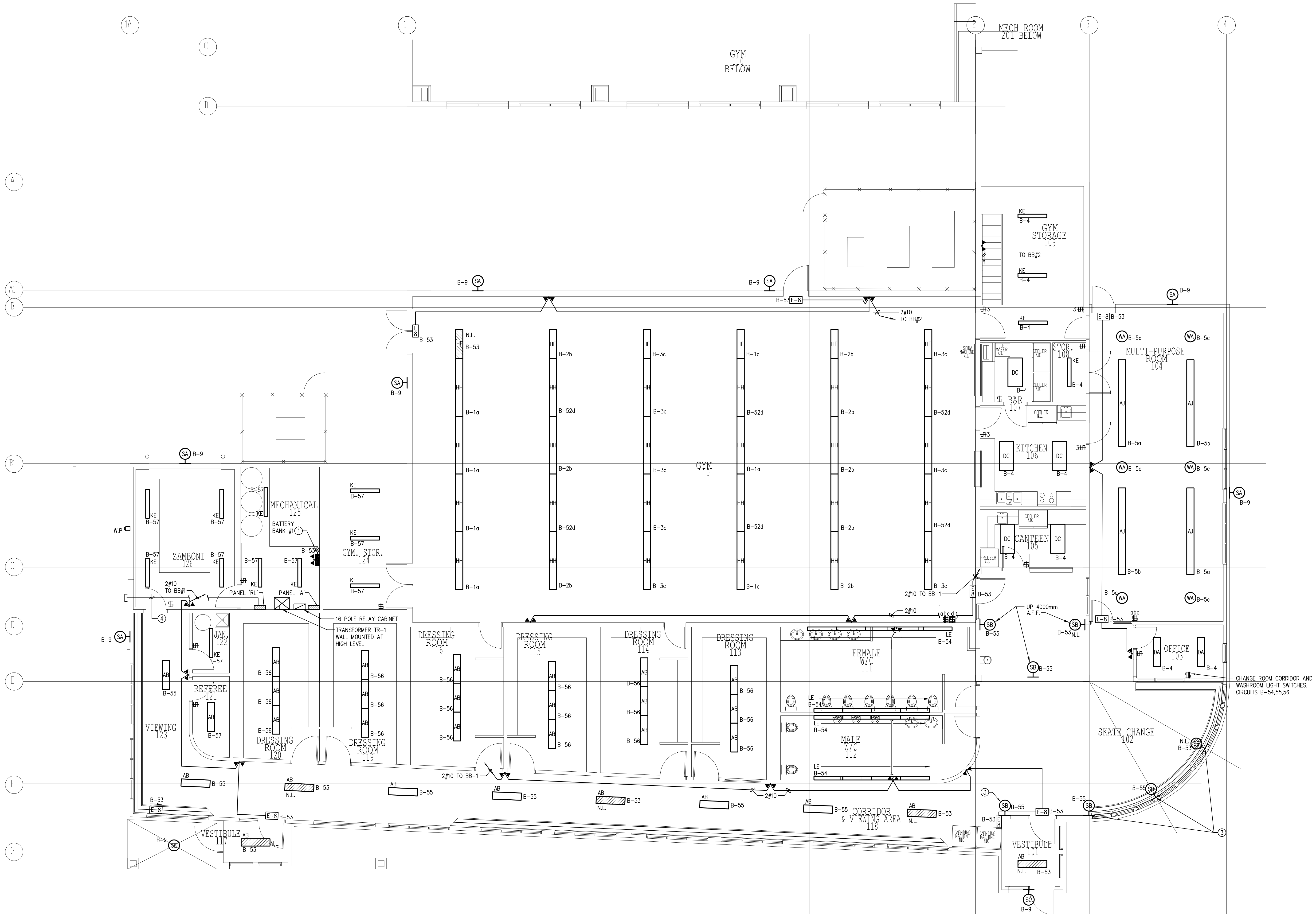
GROUND FLOOR PLAN - LIGHTING SCALE 1:75
