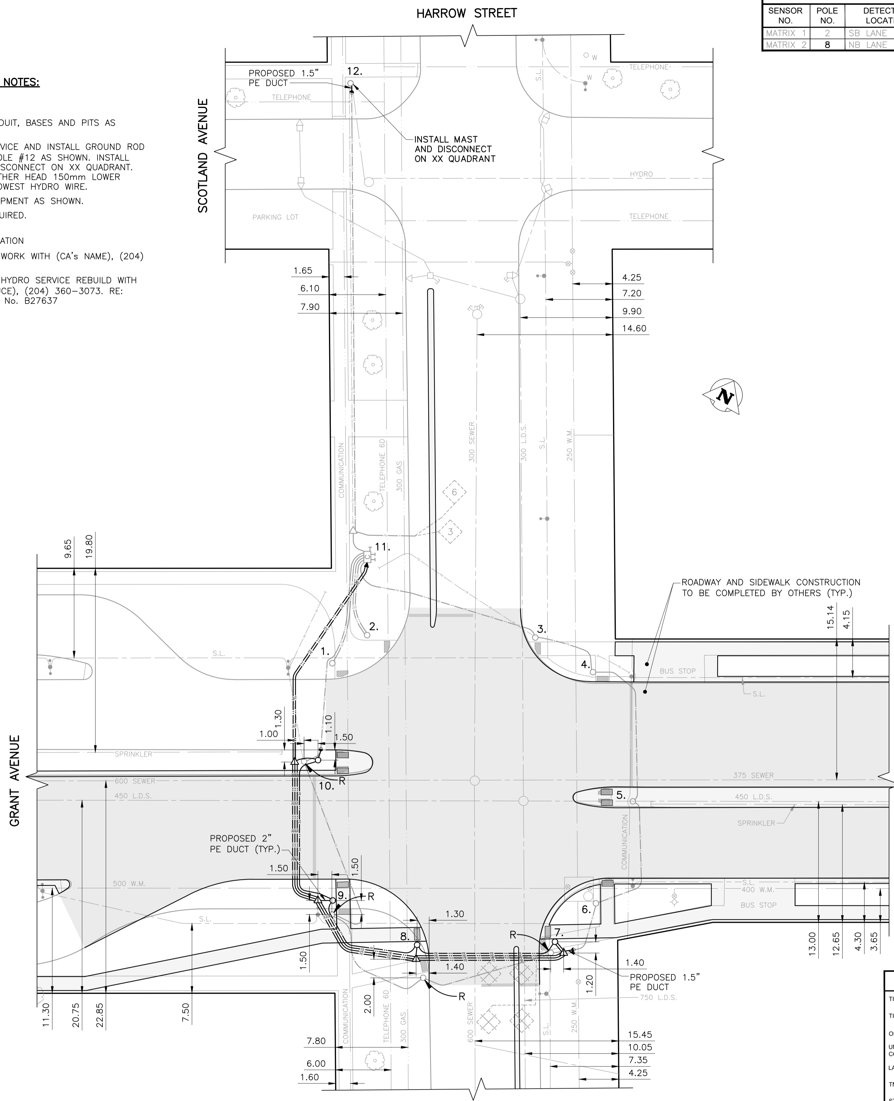
PLAN VIEW: UNDERGROUND CONSTRUCTION 1:250
