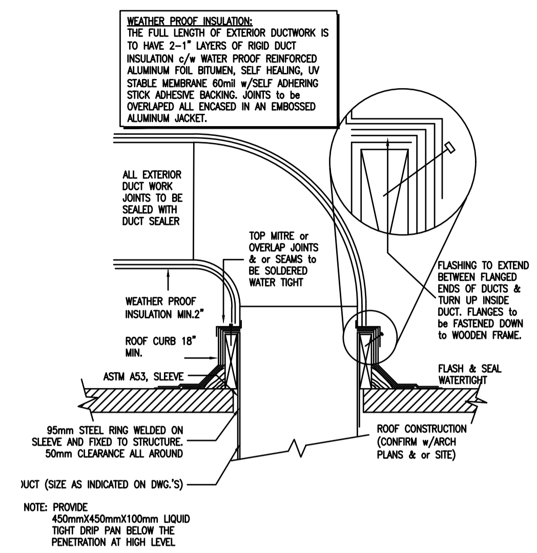
2 DUCT THROUGH ROOF DETAIL M5 NTS
