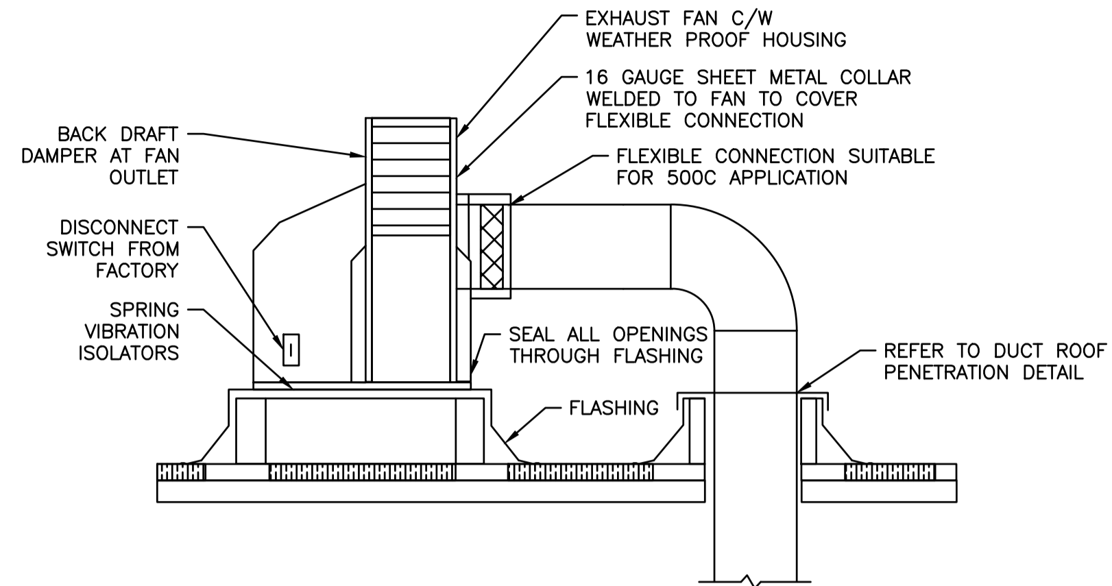
1 ROOF MOUNTED EXHAUST FAN DETAIL M5 NTS
