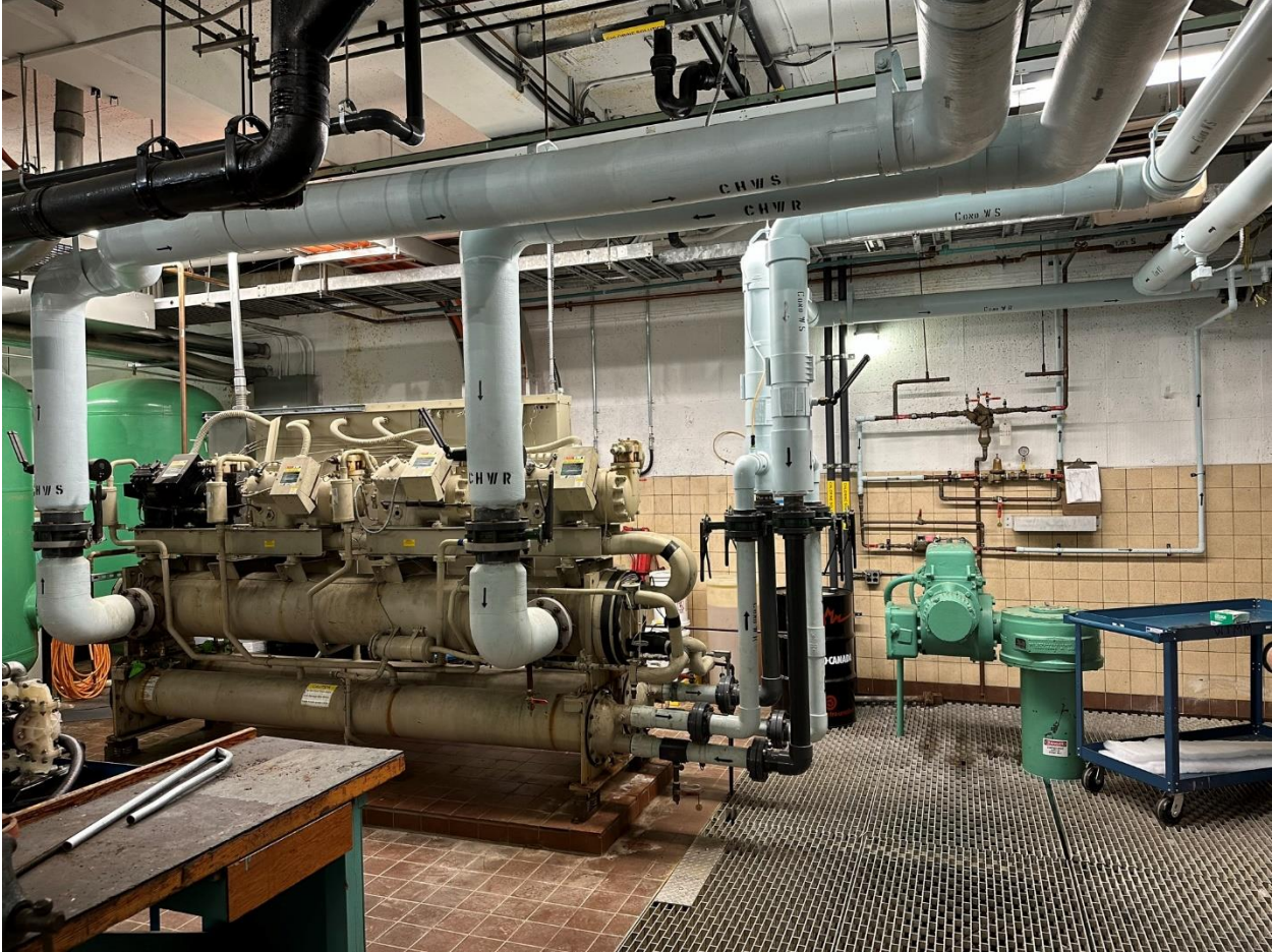
Figure 9: Existing indoor chiller, looking east.
