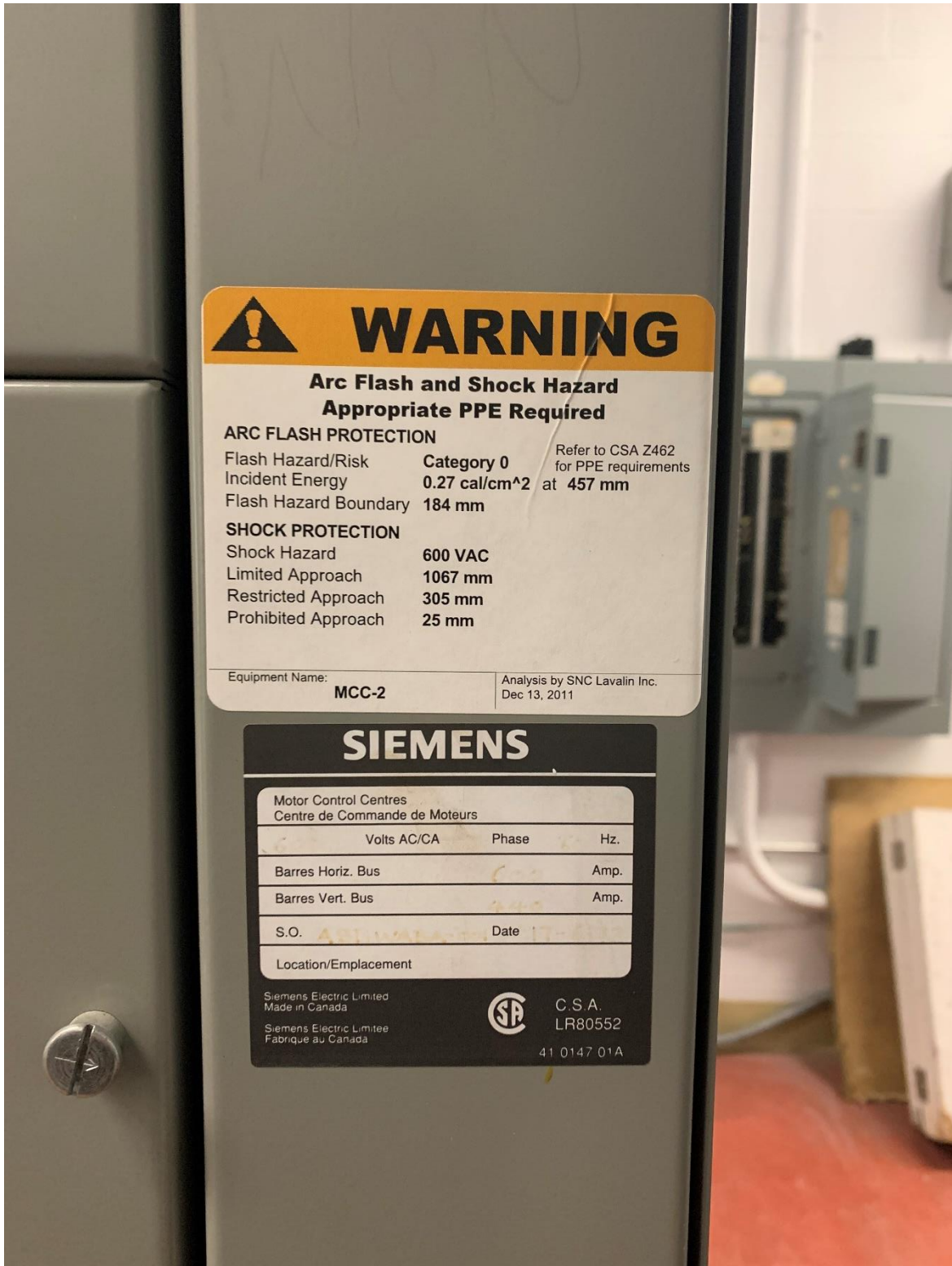
Figure 20: Existing MCC-2 labels.
