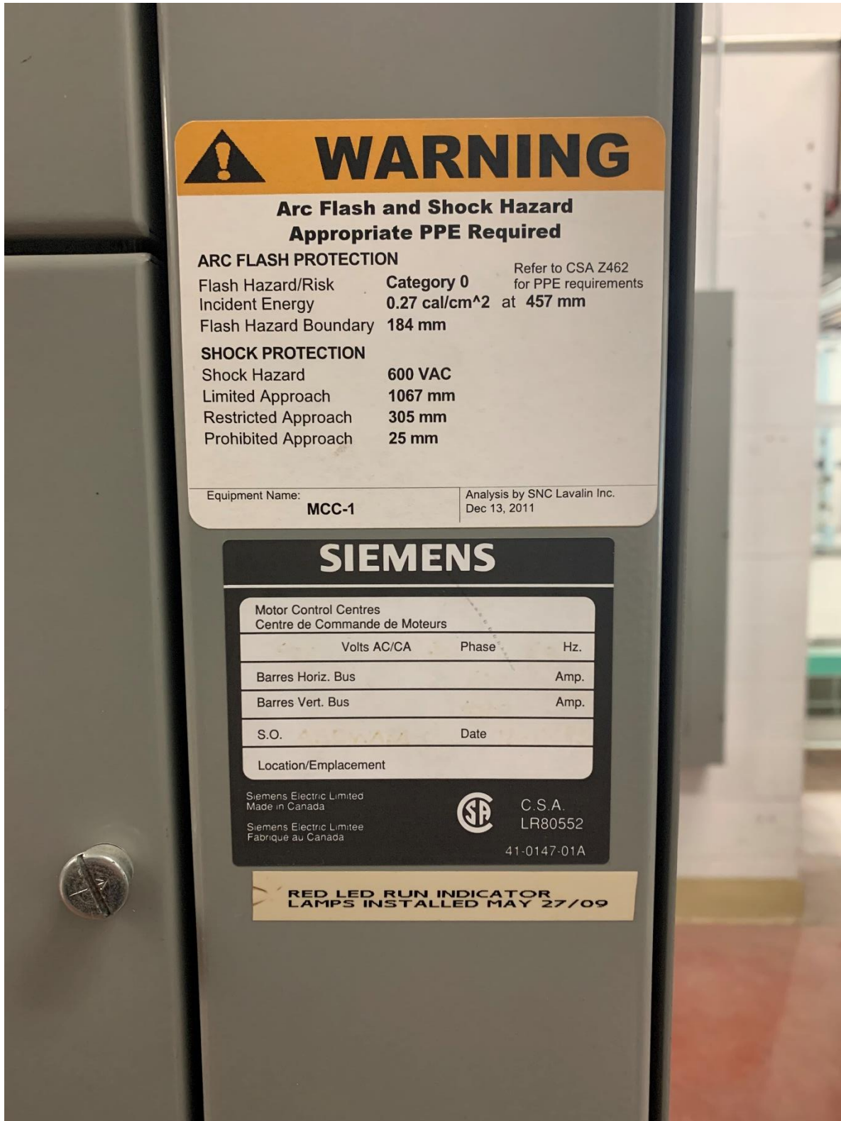
Figure 19: Existing MCC-1 labels.
