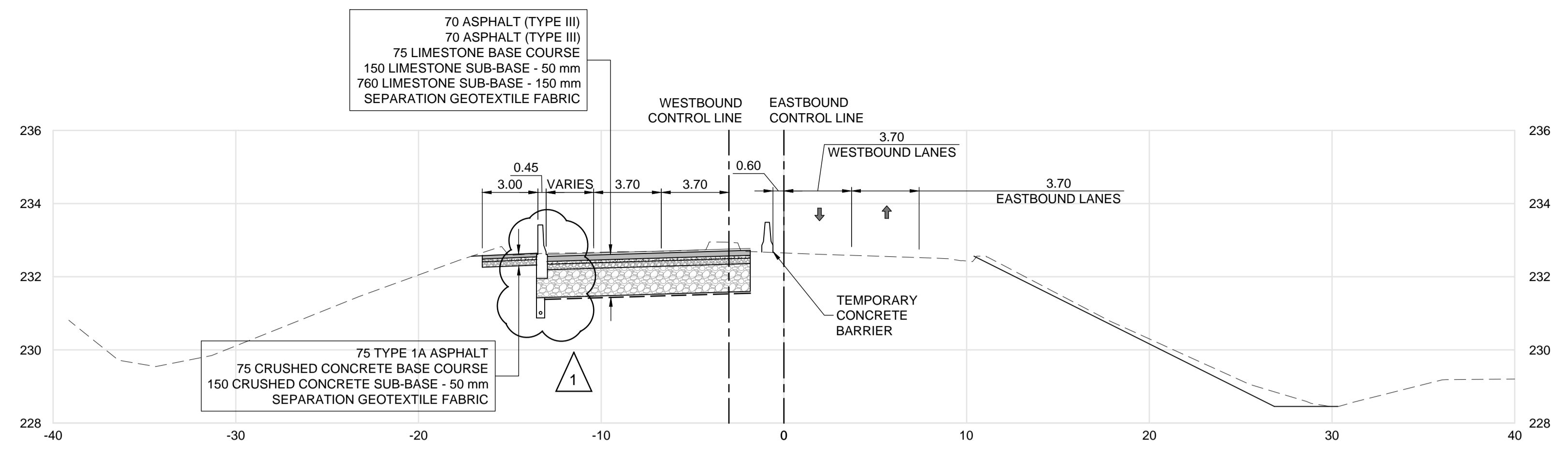
C DETOUR - STA: 5+060 (LOOKING EAST) SCALE: HORZ. 1:100 VERT. 1:50
