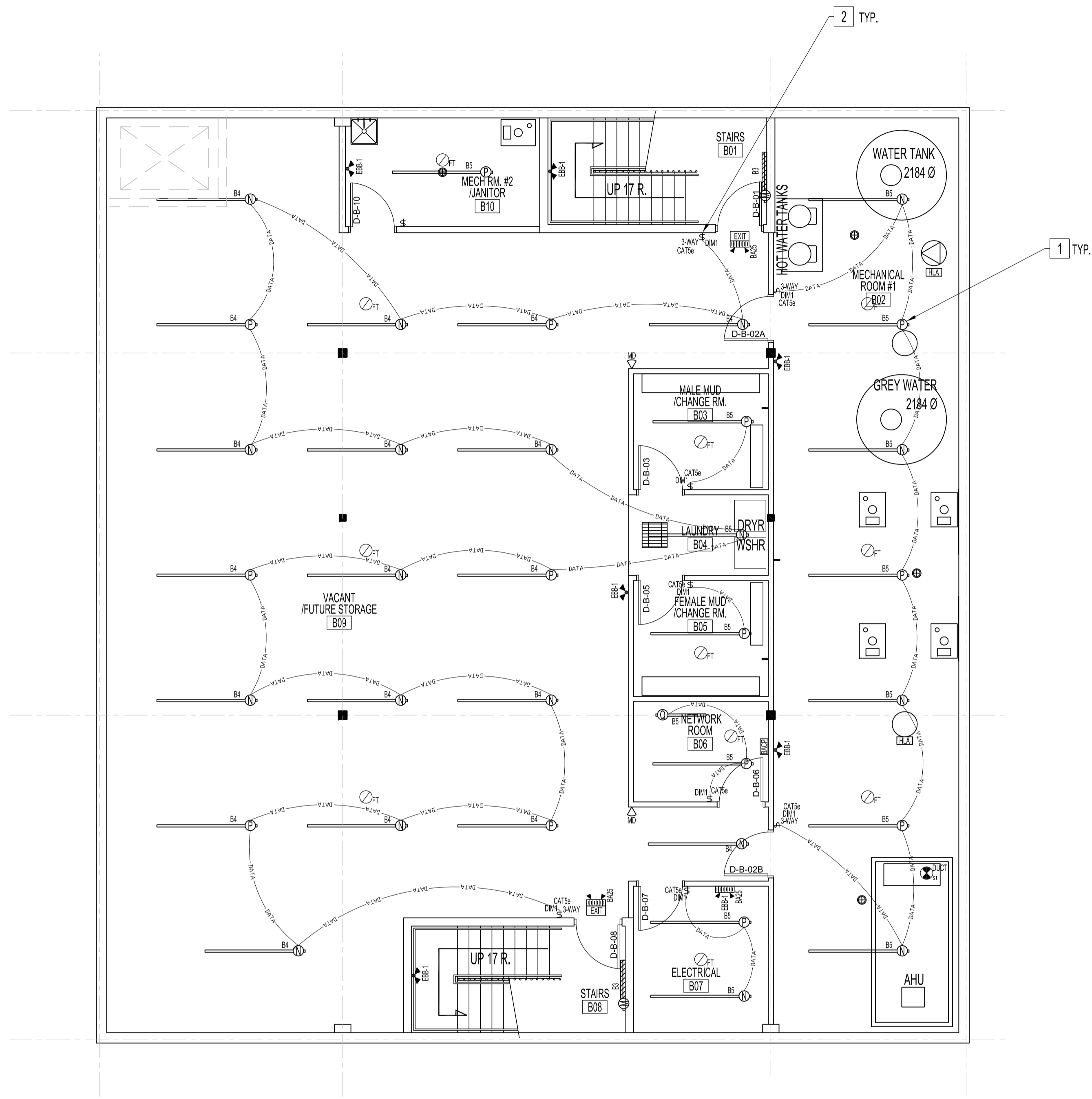
NORTH BASEMENT REFLECTED CEILING PLAN - LIGHTING SCALE 1:75
