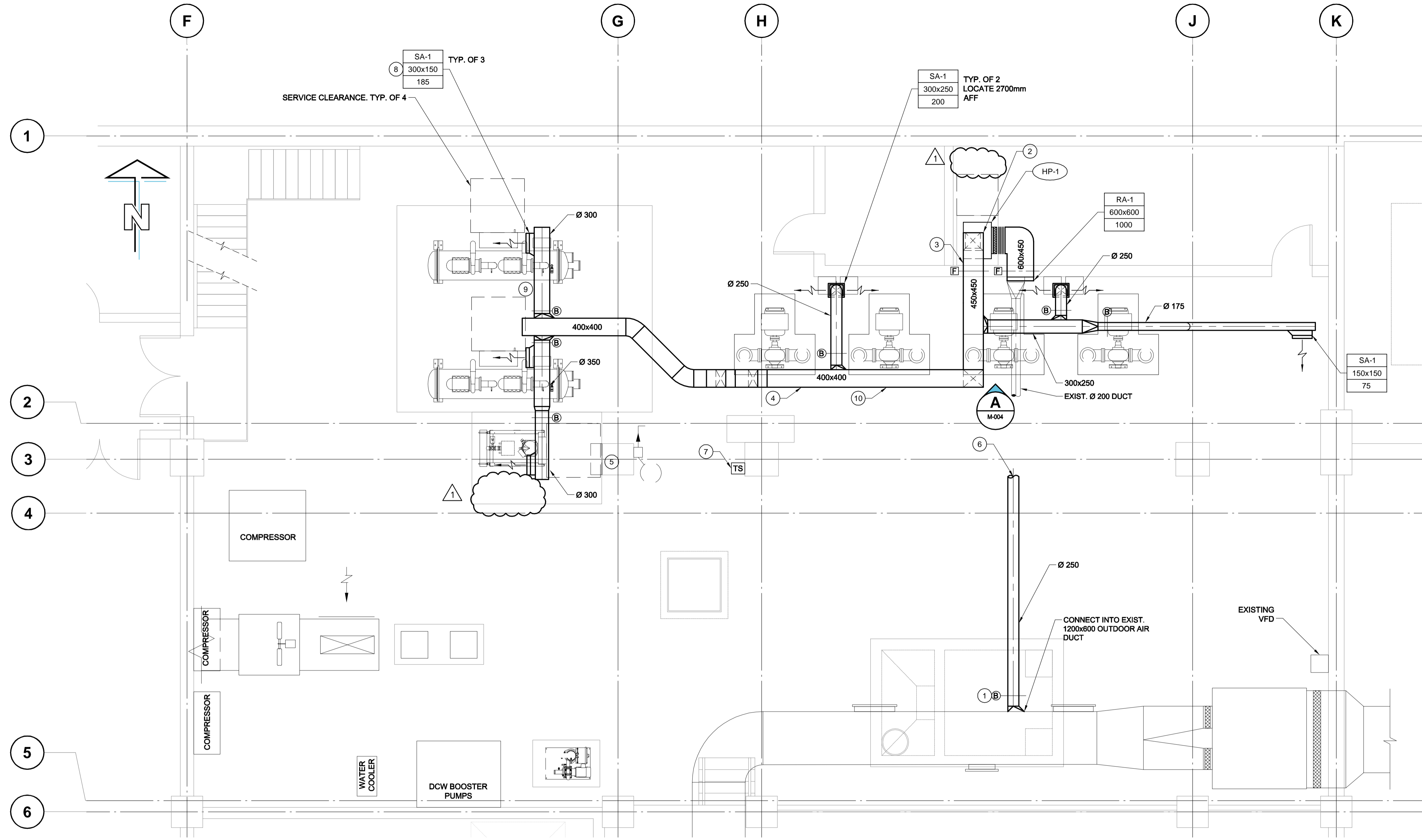
PLAN 1 SUB-BASEMENT VENTILATION SCALE 1:50 0 500 1000 1500 mm
