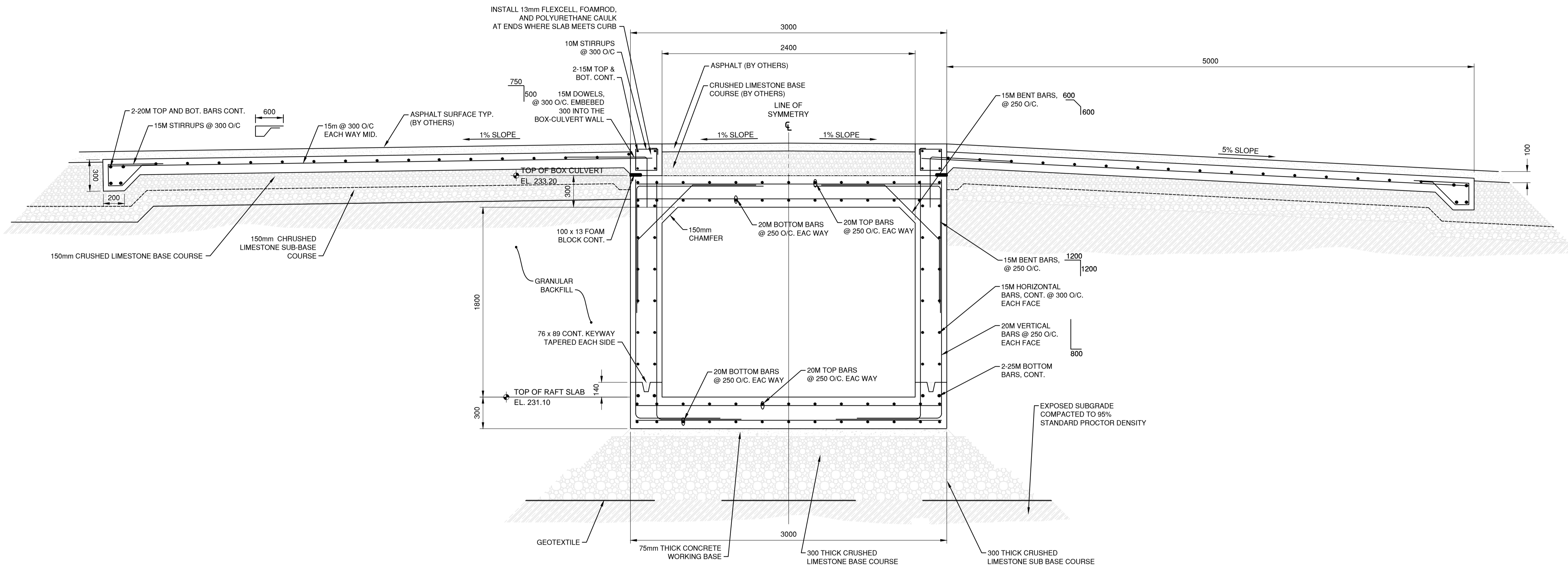
1 BOX CULVERT- SECTION 1:20
