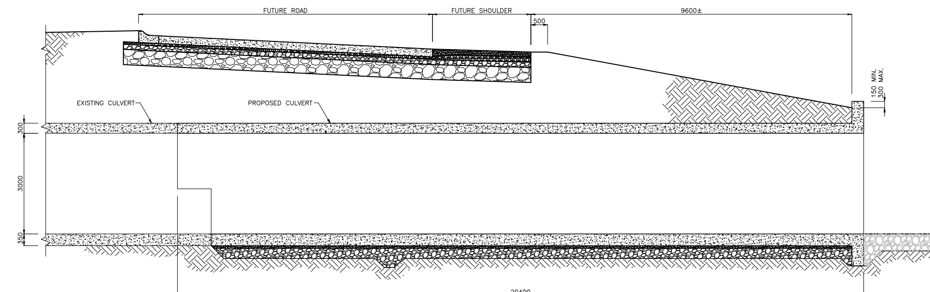
A SECTION 1:50
