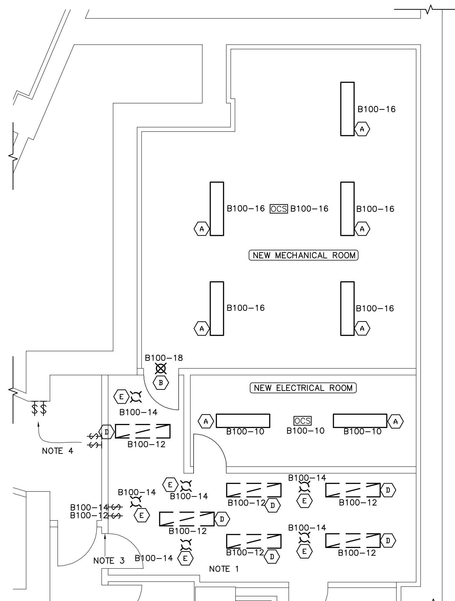
2 MECHANICAL/ELECTRICAL ROOM - LIGHTING PLAN M05 SCALE 1:50
