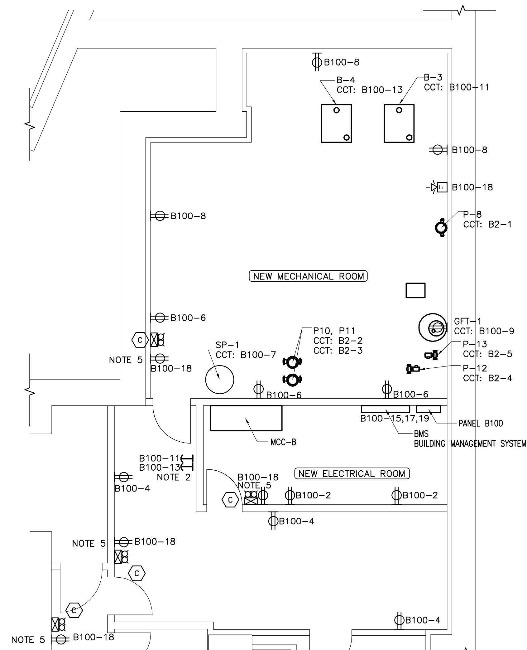
1 MECHANICAL/ELECTRICAL ROOM - DISTRIBUTION PLAN M05 SCALE 1:50
