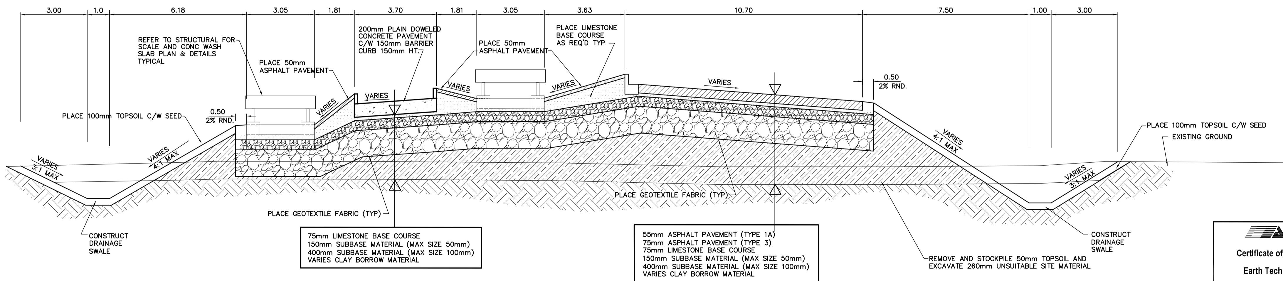
3 PAVEMENT SECTION C1.03 SCALE H=1:100 V=1:33
