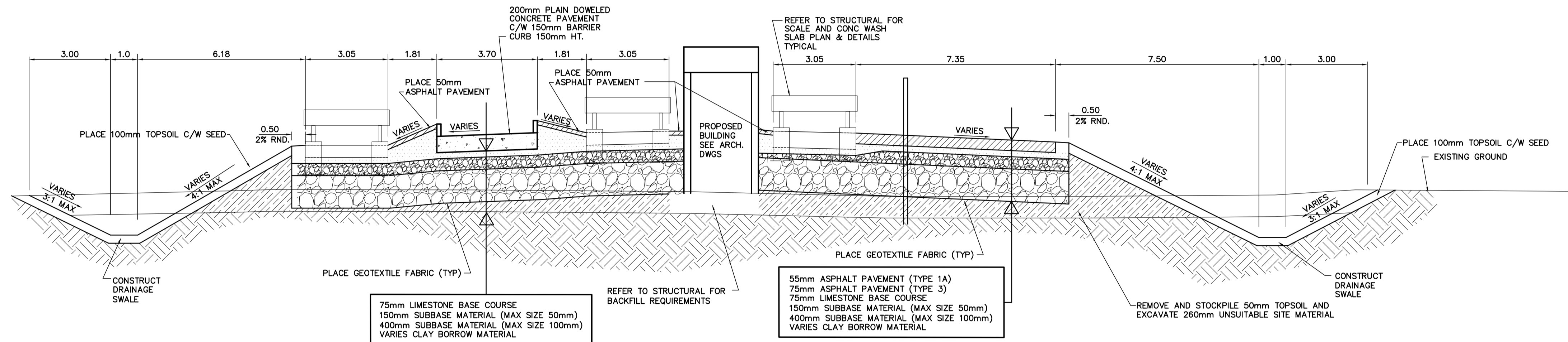
2 PAVEMENT SECTION C1.03 SCALE H=1:100 V=1:33
