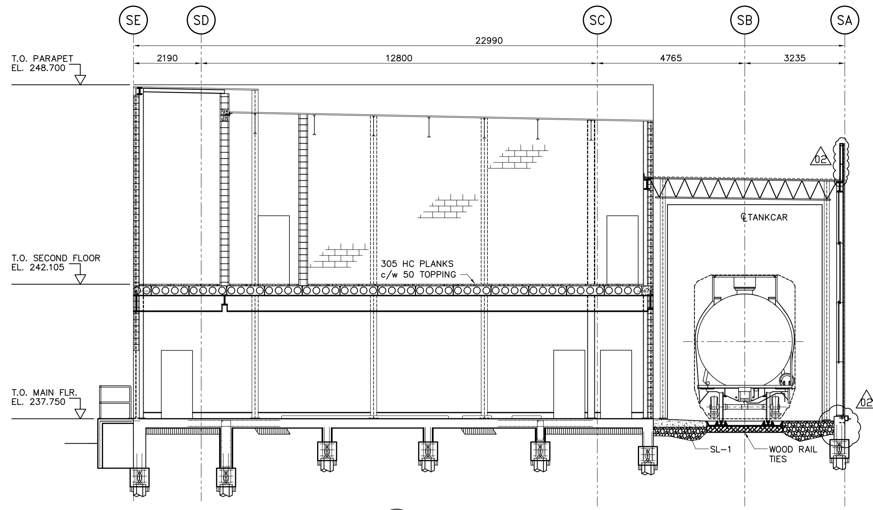
8 SECTION WS-S0203 1:75
