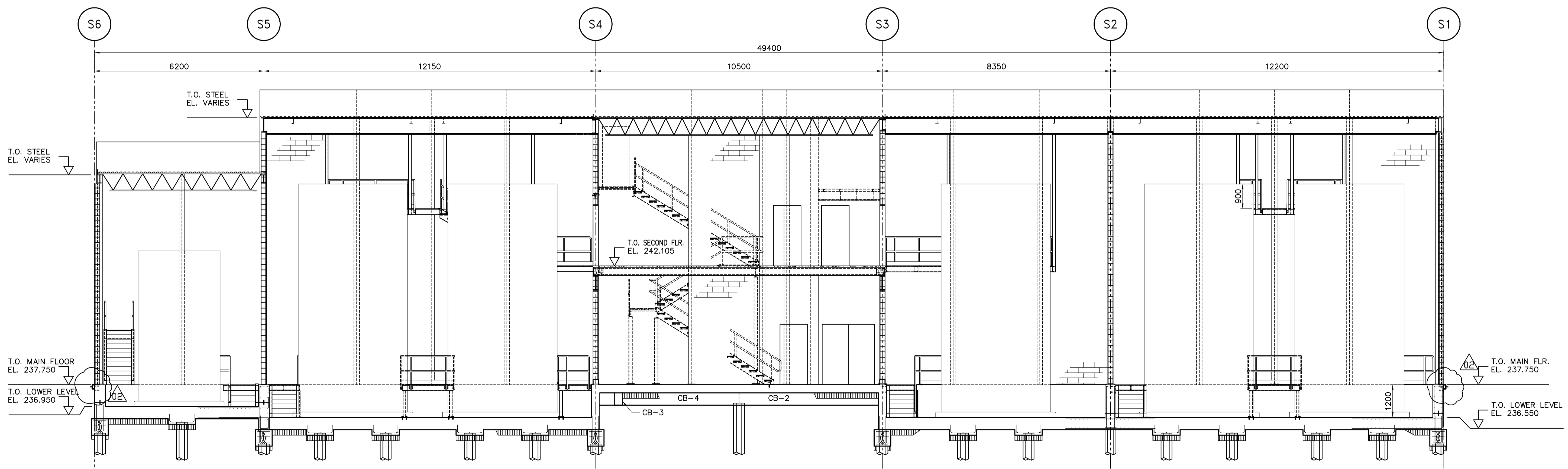
9 SECTION WS-S0203 1:75
