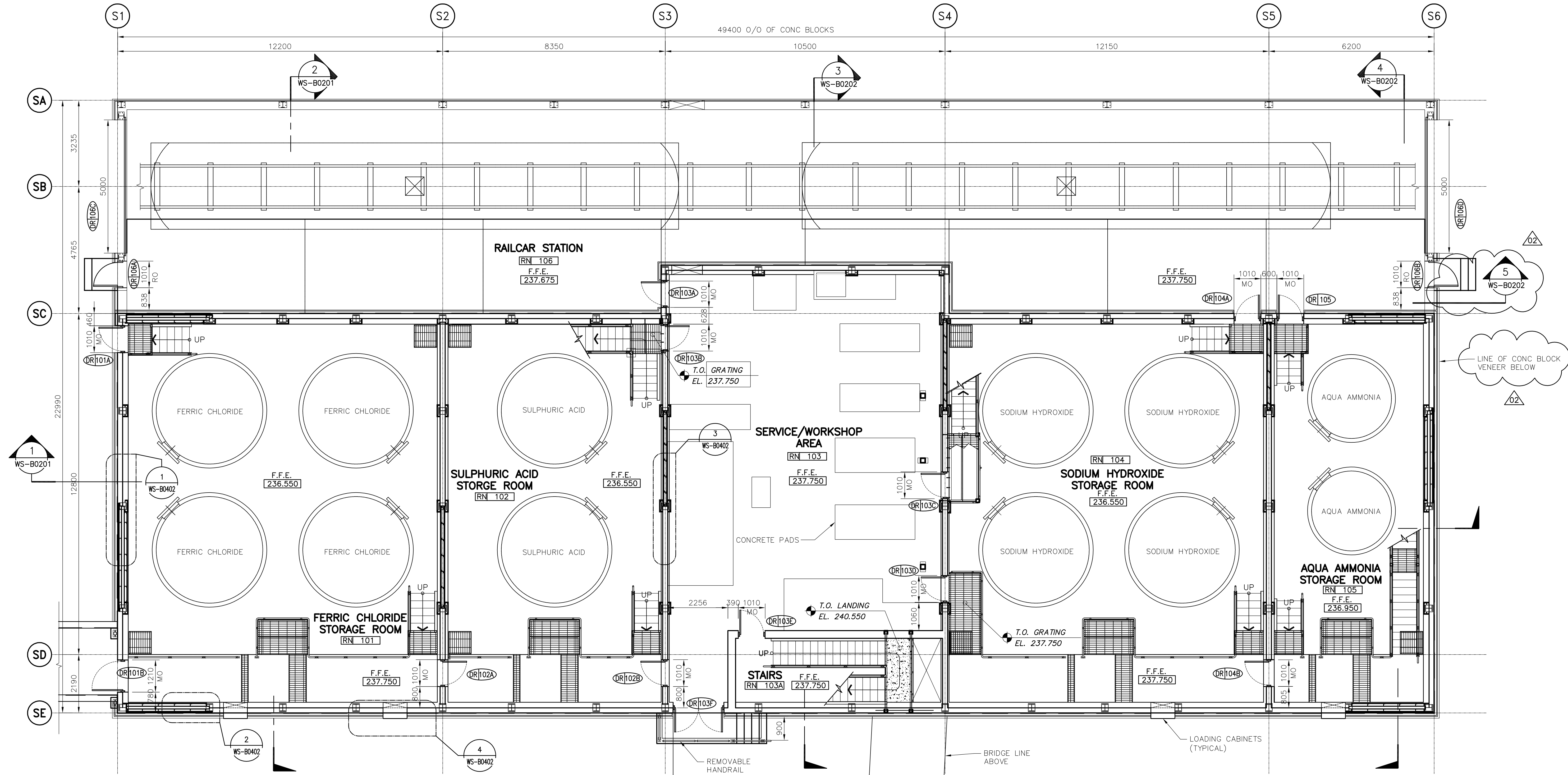
1 MAIN FLOOR PLAN WS-B0110 1:75
