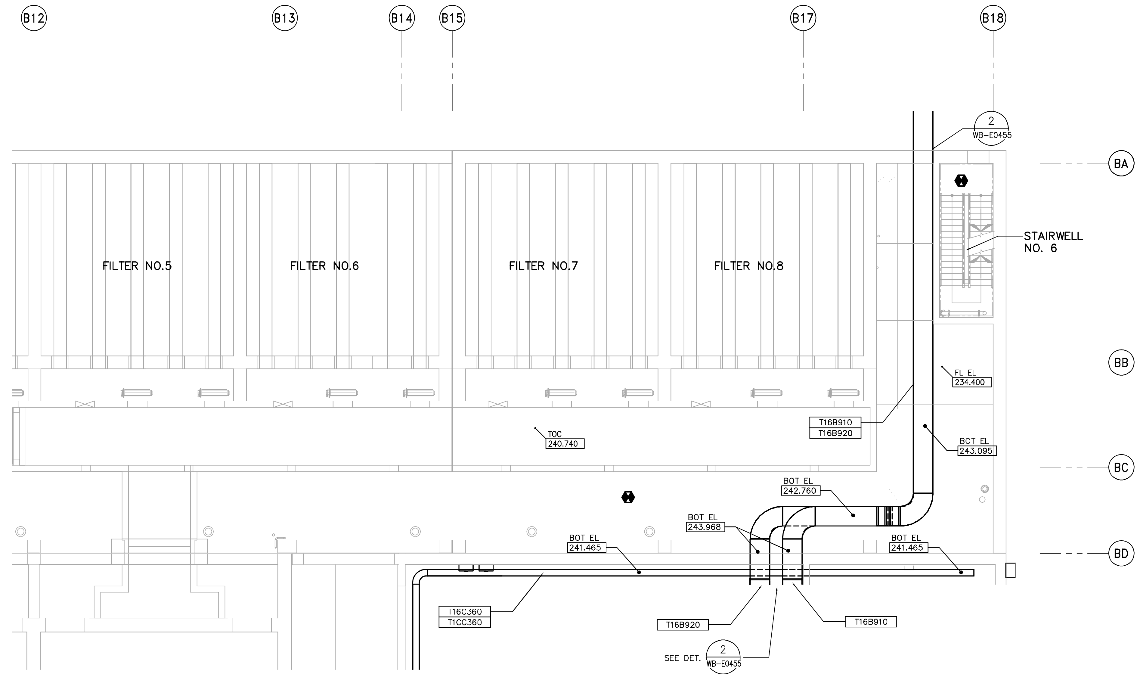
SECOND FLOOR FACILITY PLAN (AREA 2) 1:100
