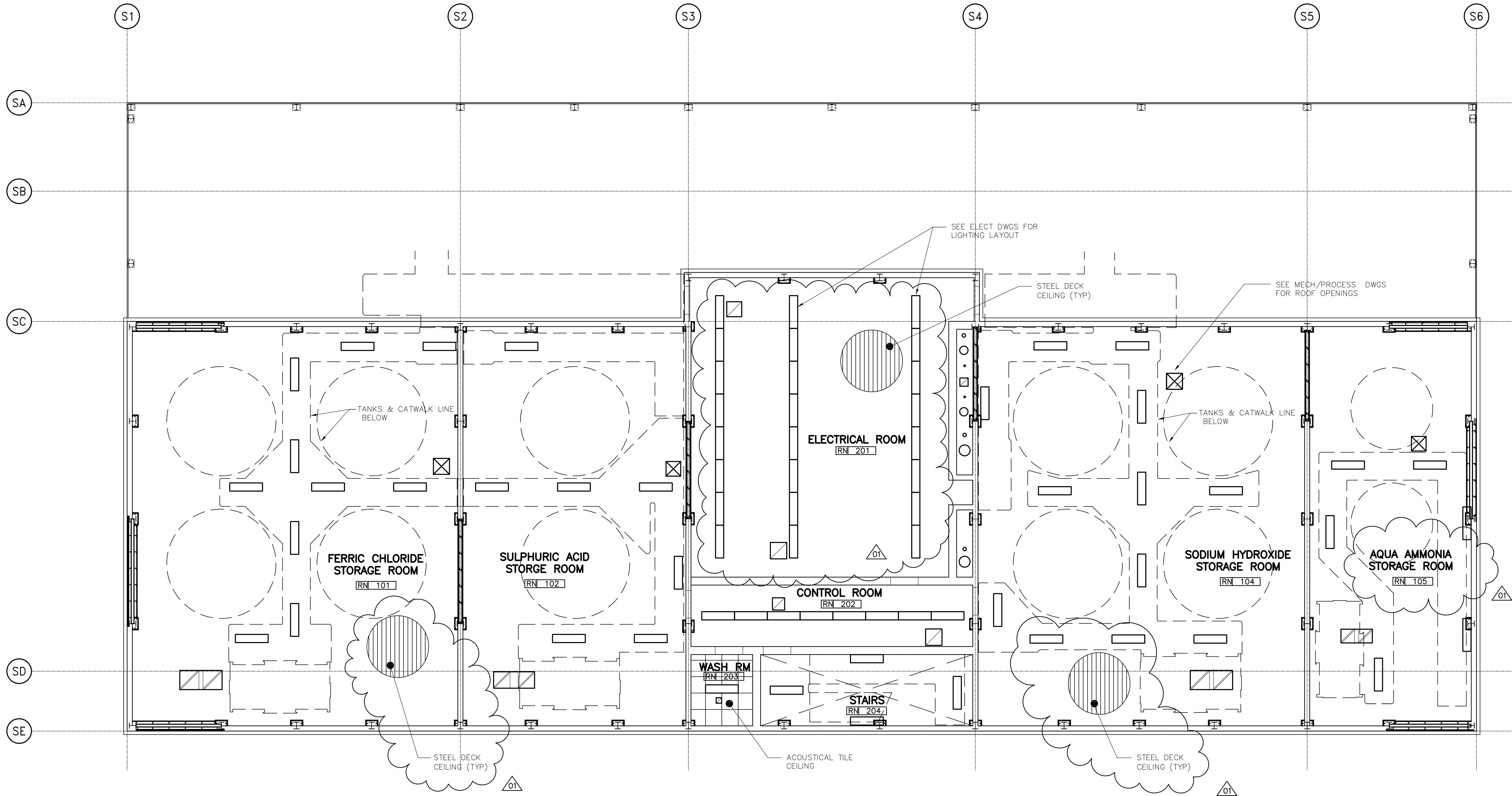
1 SECOND FLOOR REFLECTED CEILING PLAN WS-B0122 1:75
