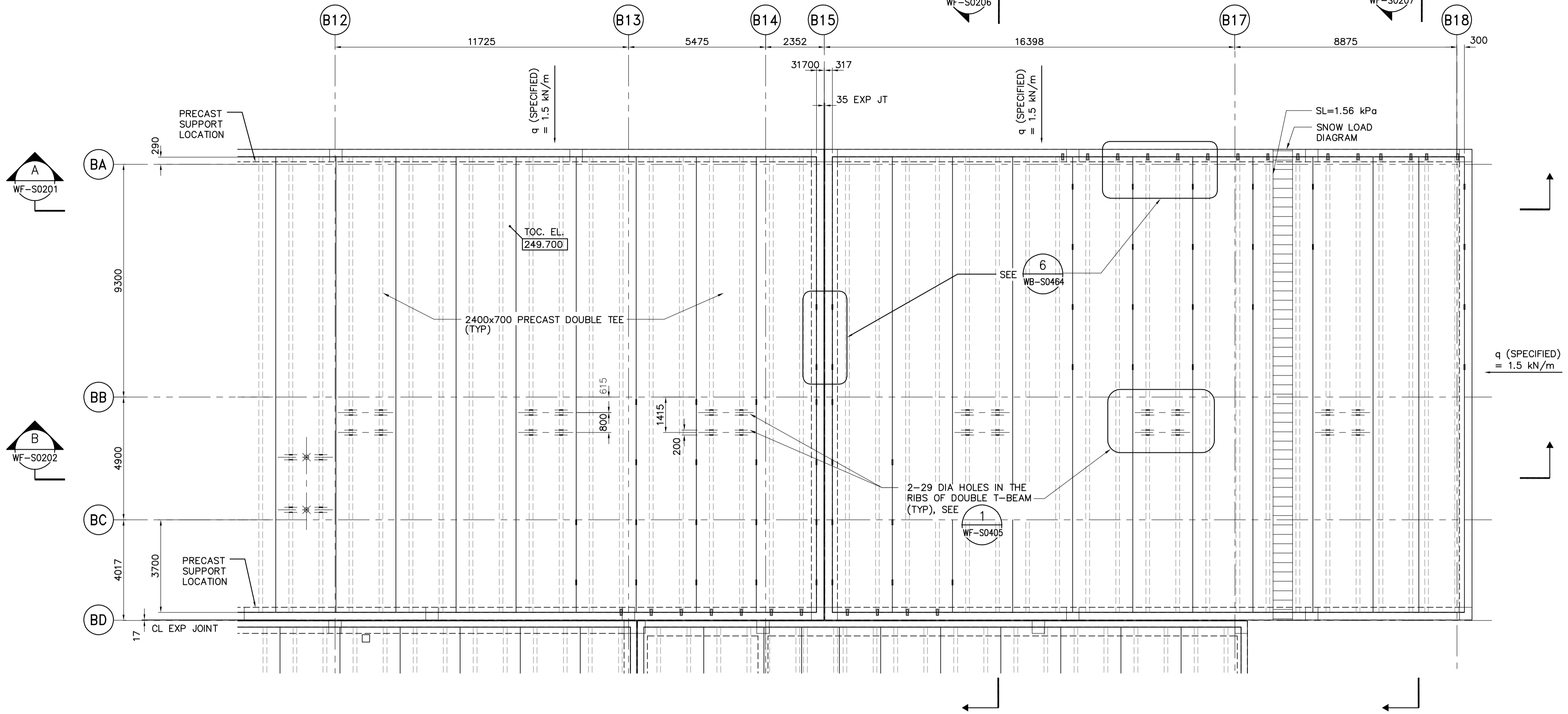
ROOF PLAN 1:100
