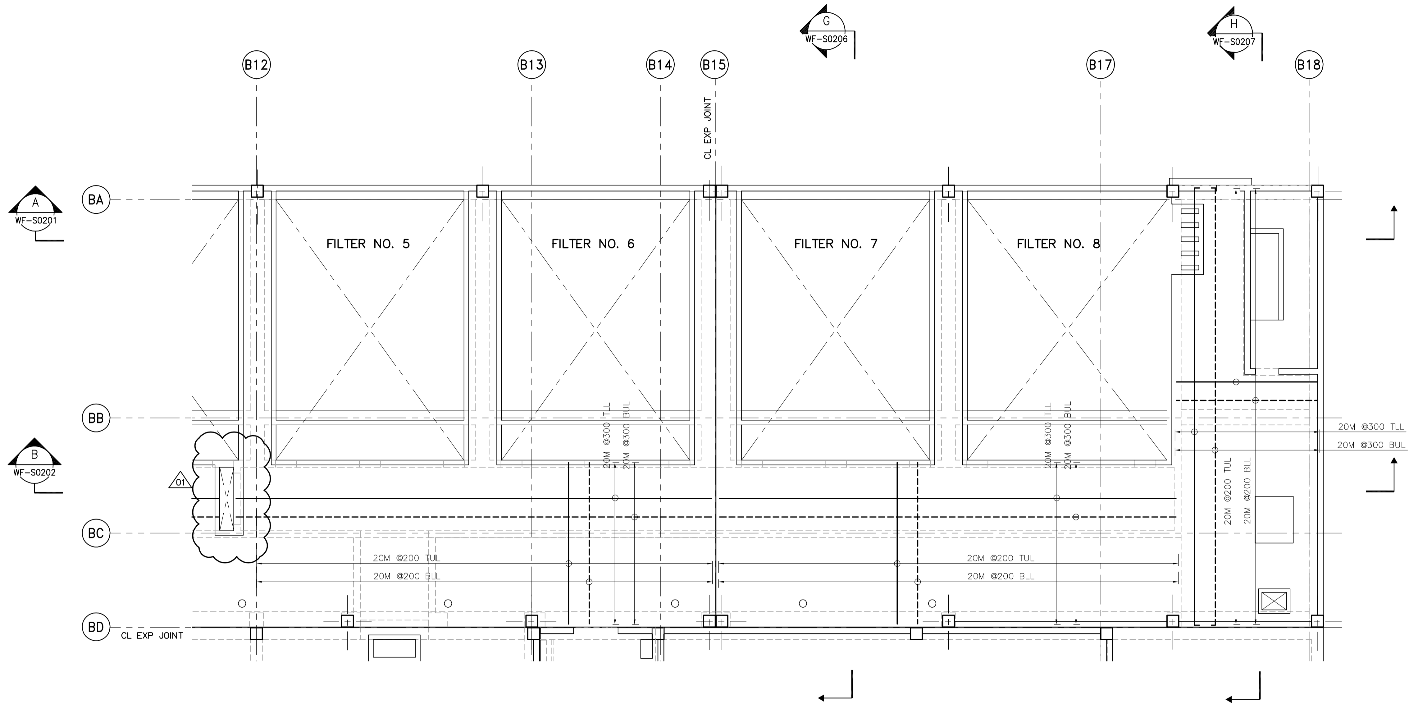
THIRD FLOOR PLAN AT EL 245.000 1:100
