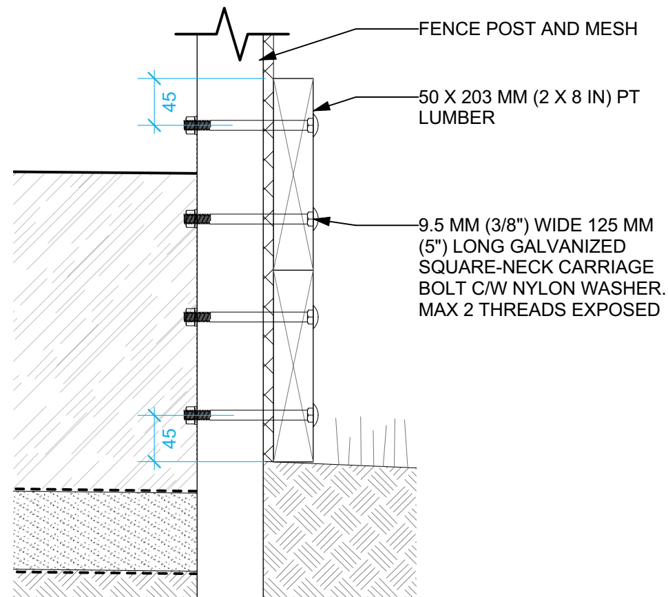
2 LUMBER EDGING TO FENCE ATTACHMENT Scale: 1:5
