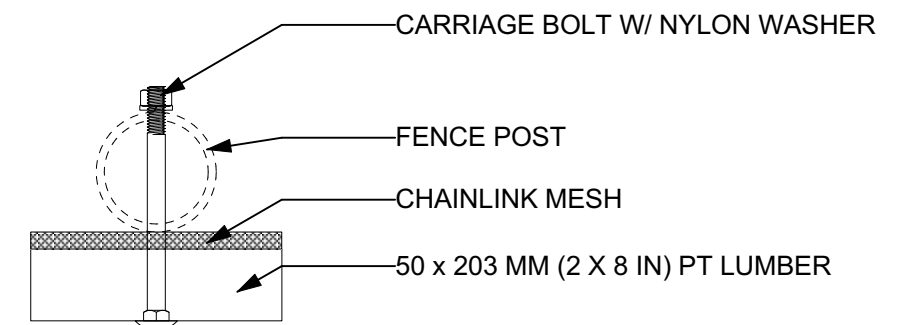
3 LUMBER EDGING TO FENCE ATTACHMENT 2 Scale: 1:4
