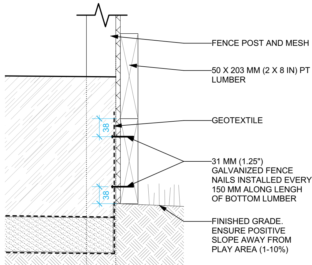
1 LUMBER EDGING WITH FABRIC Scale: 1:5
